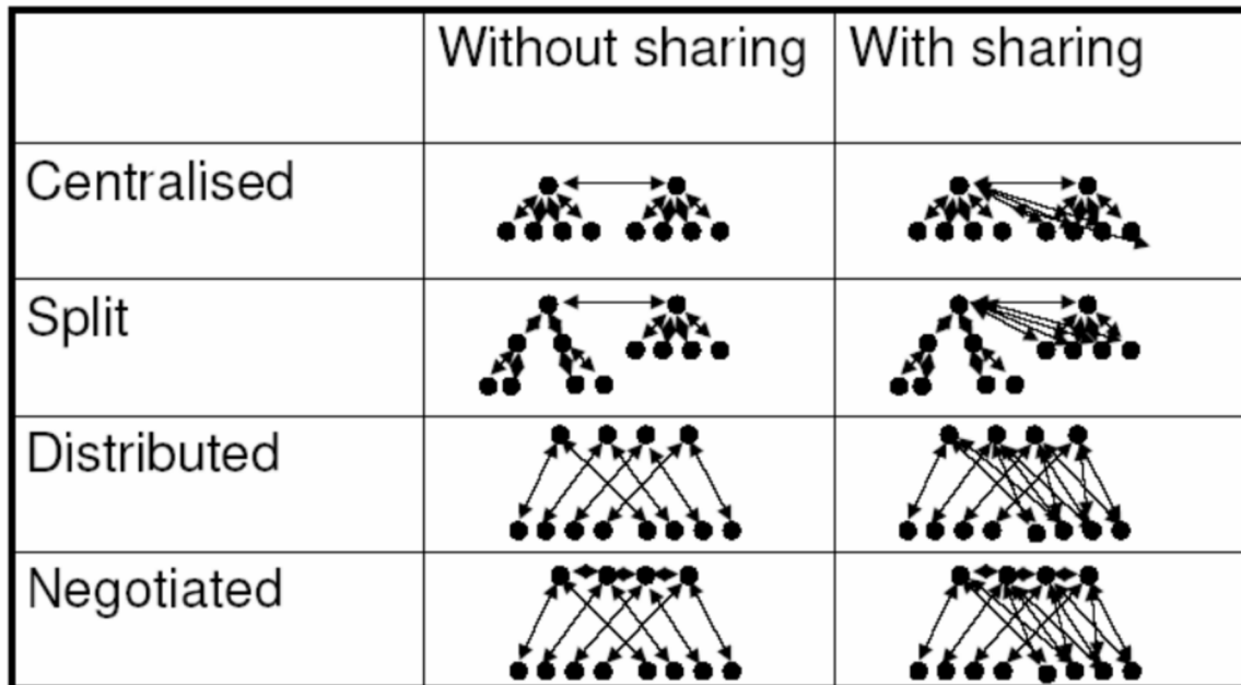
Figure 2. Dekker network architectures
